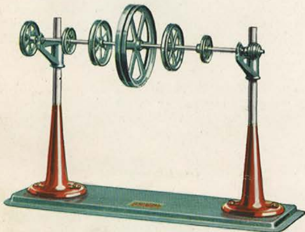
No. 975—7-Pulley ADJUSTABLE COUNTERSHAFT. 6 single and one 2 speed pulley. Adjustable brackets. Uprights 8" tall. Finished in red and battleship gray ZAPON lacquer enamel.
