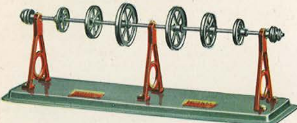
No. 970—8-Pulley Countershaft. A wonderful value. 6 single and 2 two speed pulleys. Three uprights maintain rigid alignment. Finish and style similar to No. 960. Height 4 \frac{3}{4} ". Length 12 \frac{3}{4} ". Shipping wt. 2 lbs.
