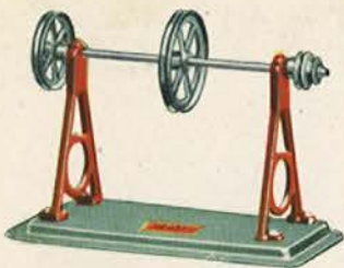
No. 960—3-Pulley Countershaft. 2 single, one double pulley. Rigidly mounted on heavy gauge metal base. Finished in red and battleship gray. ZAPON lacquer enamel. Height 4 \frac{3}{4} ". Length 6". Shipping wt. 1 lb.
